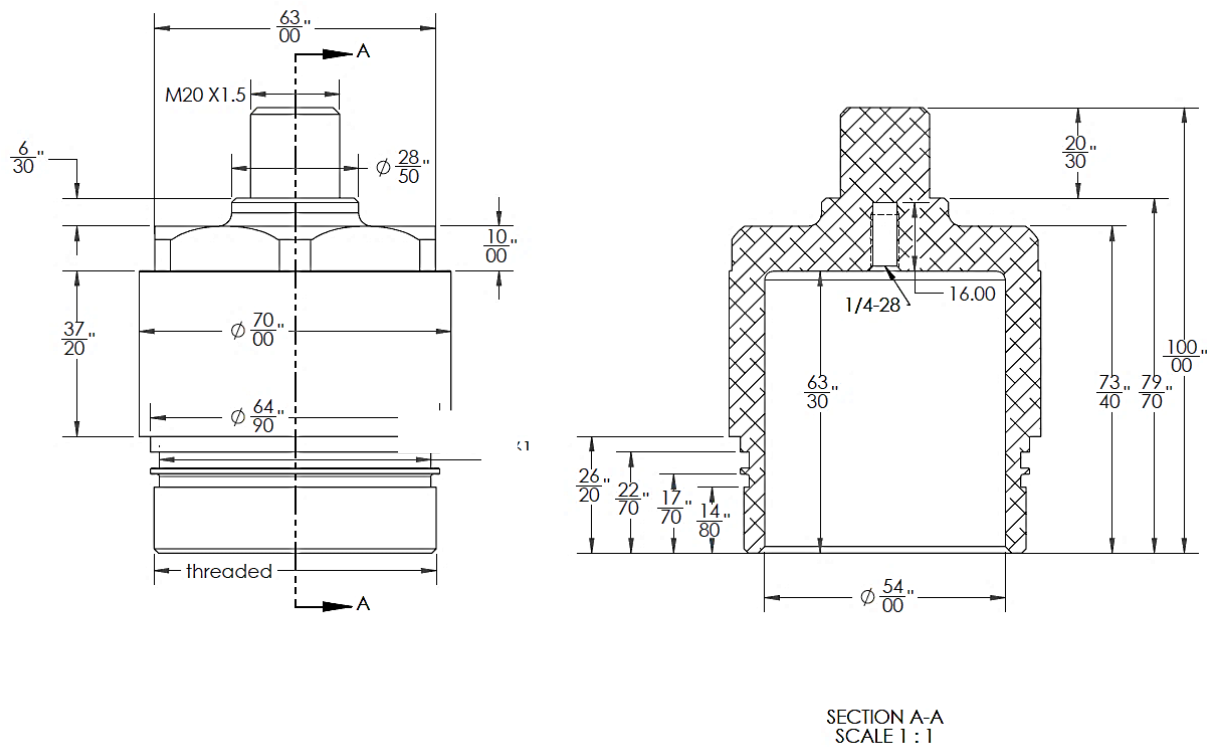
Figure 1. Yekan YB/21128 Velocity Transducer Housings Top Diagram
