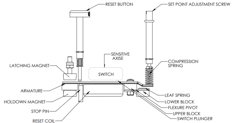
Figure 1. MS60 Mechanism
