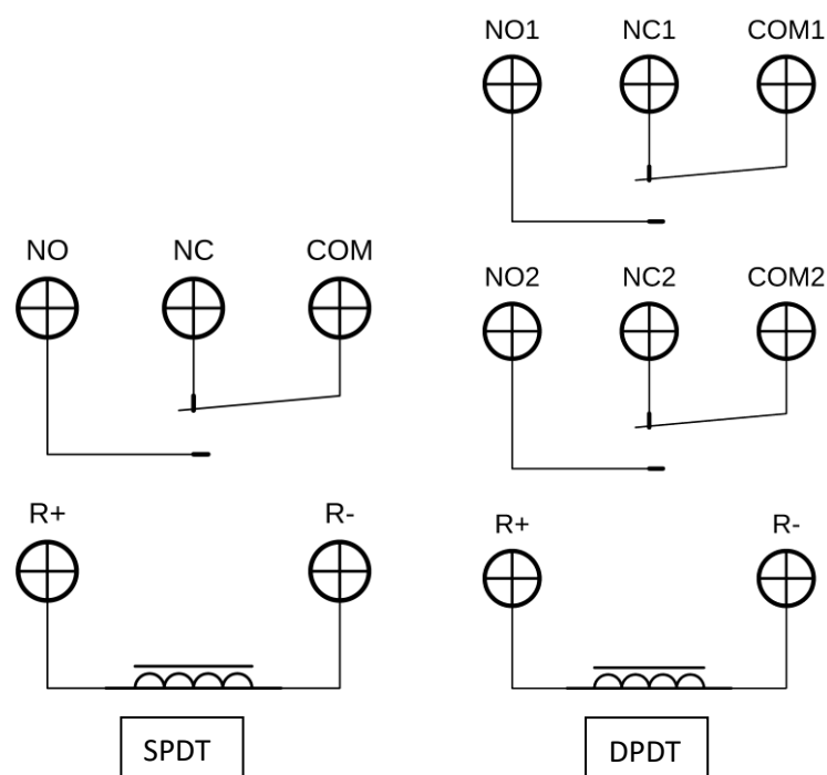
Figure 4. Wiring connections
