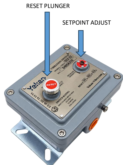
Figure 2. MS60 setpoint adjustment and manual reset Mechanism
